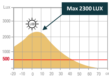
Measurement in Lux on the worktop in profile view at 35 cm:
