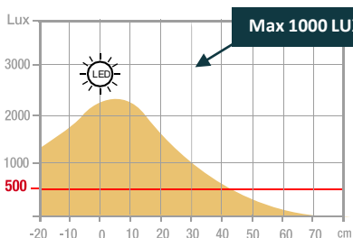
Measurement in Lux on the worktop in profile view at 35 cm:
