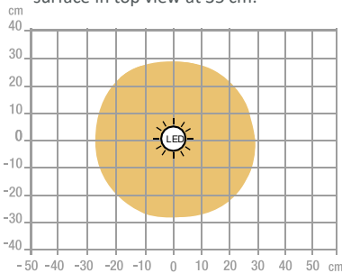
Lux measurement on the work surface in top view at 35 cm:
