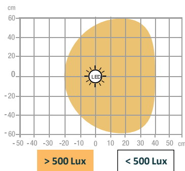
Measurement of Lux on the worktop in 40 cm top view:
