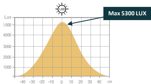
Lux measurement upwards 55 cm from the light source:
